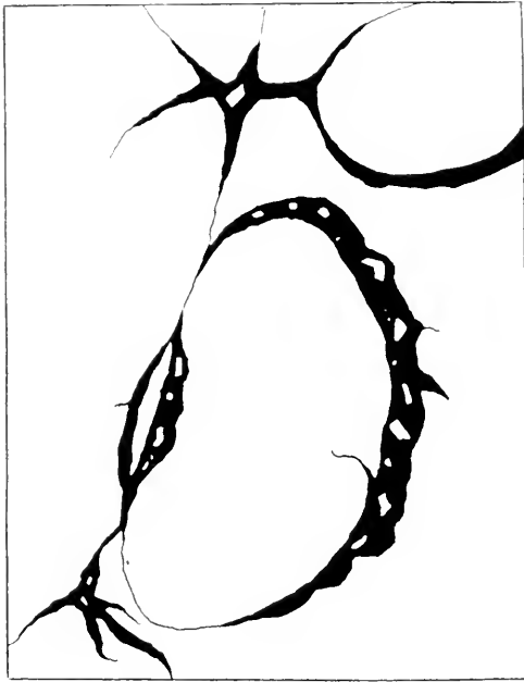
Fig. 17—Showing character of ore at Cream Hill mine, second level, Sudbury area, Ontario. White represents greenstone; black represents ore. The width of the face indicated in drawing is 15 feet.
